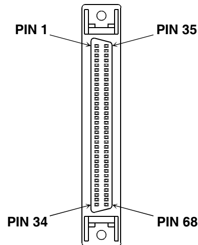
FIGURE 2-2: J200, J201, AND J202 PIN LOCATIONS
